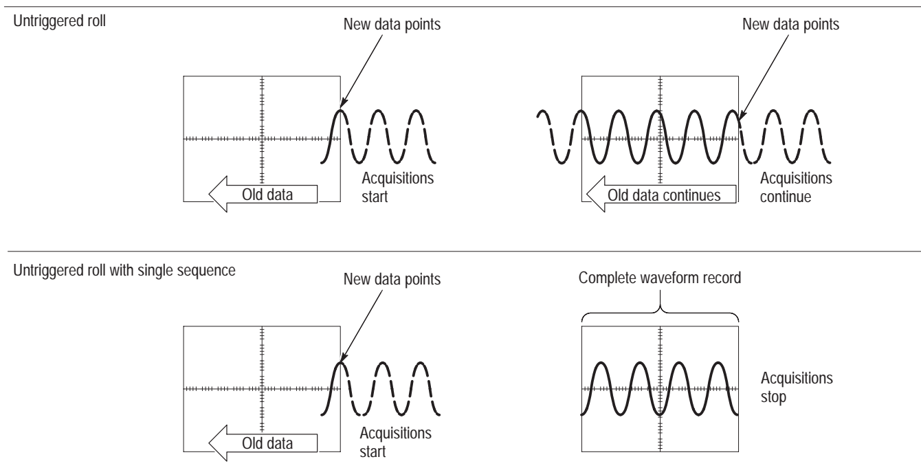
Figure 3–6: Roll mode
