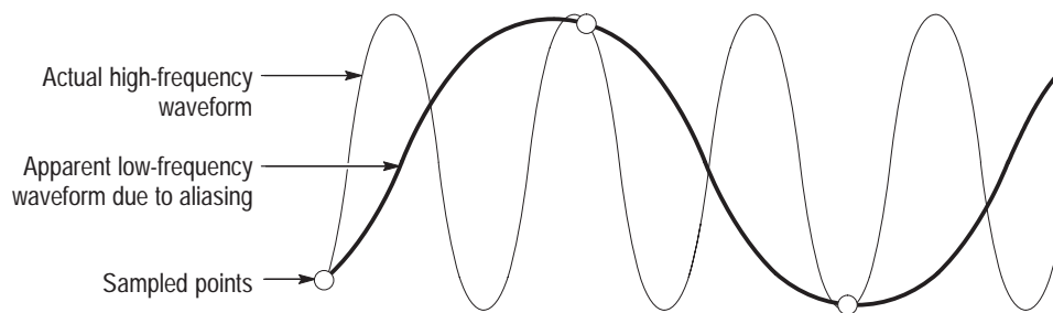
Figure 3-7: Aliasing
