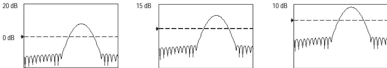
Figure 3–44: Effects of adjusting the reference level
