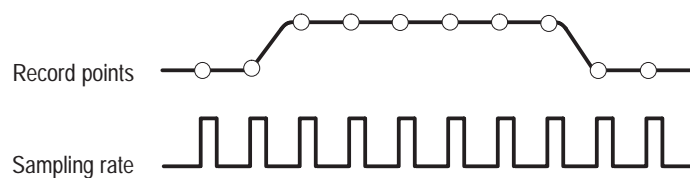
Figure 3–11: Real-time sampling
