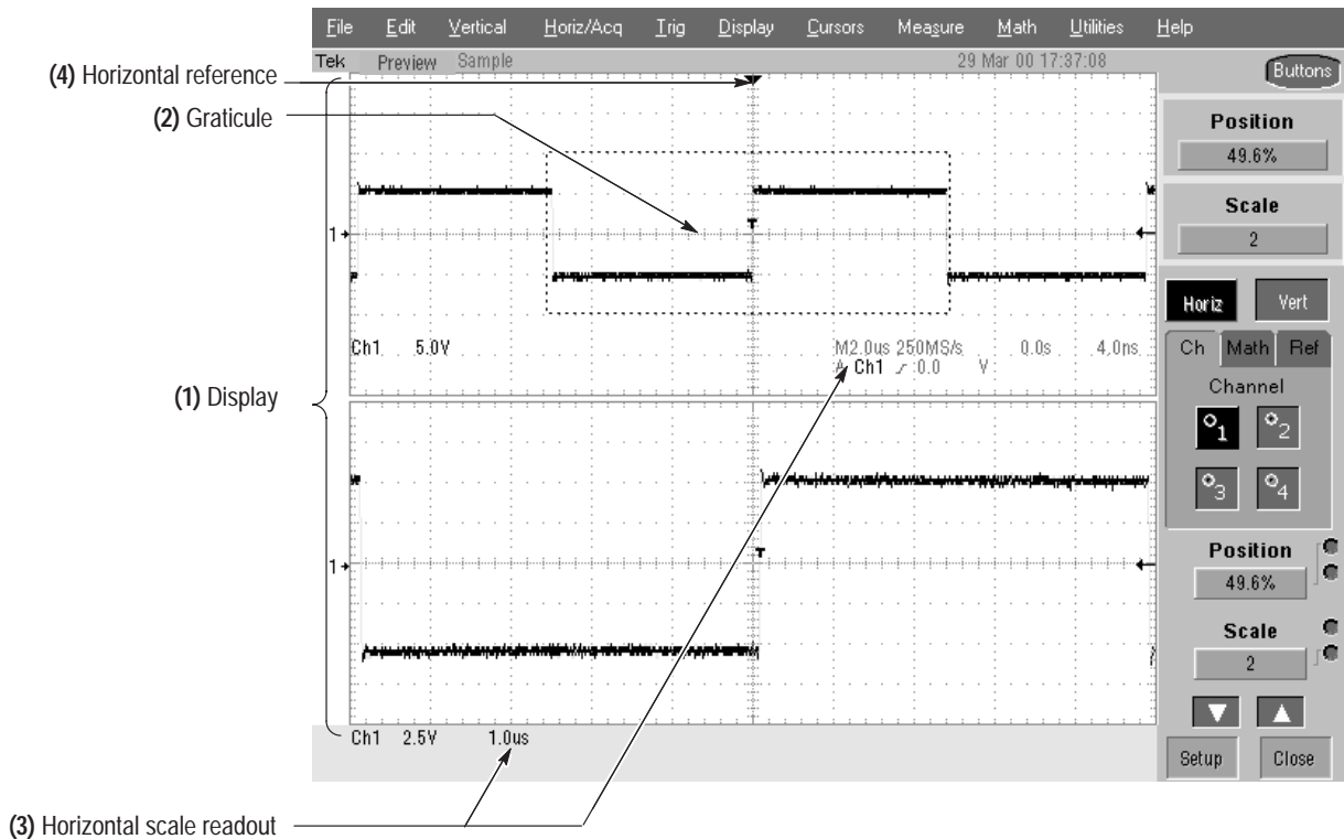
Figure 3–28: Display elements
